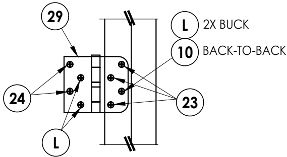
HINGE DETAIL
